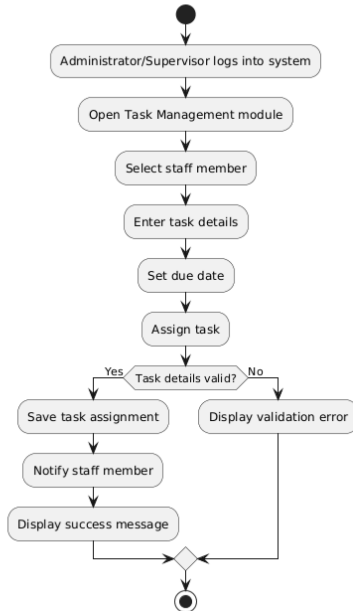
Figure 29 Activity Diagram – Assign Task
