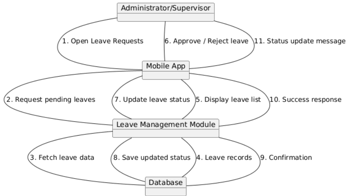
Figure 56 Collaboration Diagram for Approve / Leave Reject
