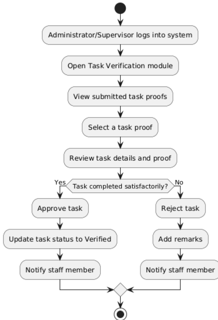
Figure 30 Activity Diagram – Verify Task
