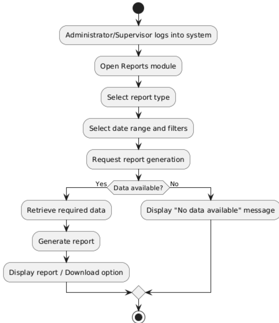
Figure 32 Activity Diagram – Generate Reports
