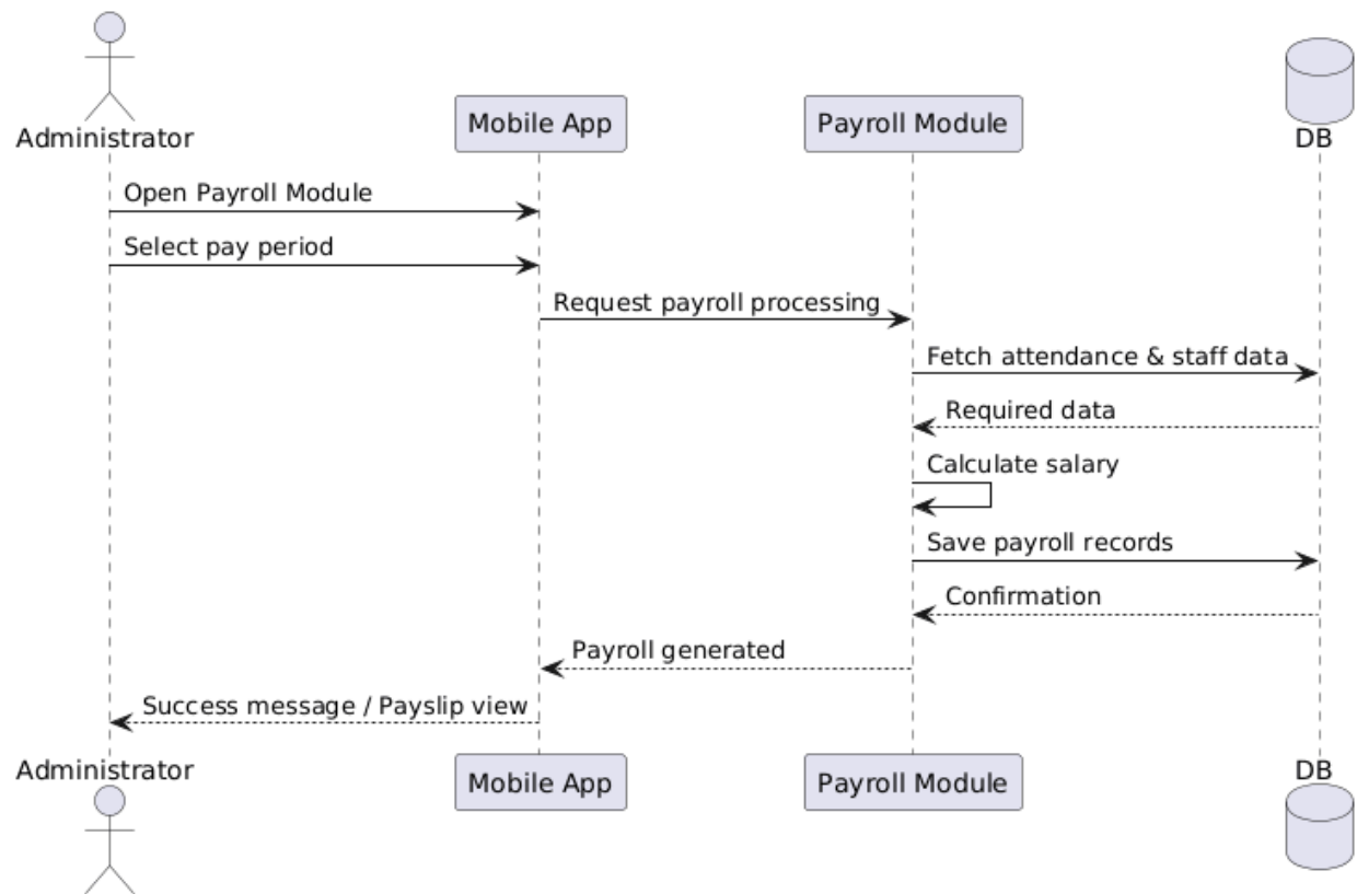
Figure 45 Sequence Diagram for Manage Payrolls
