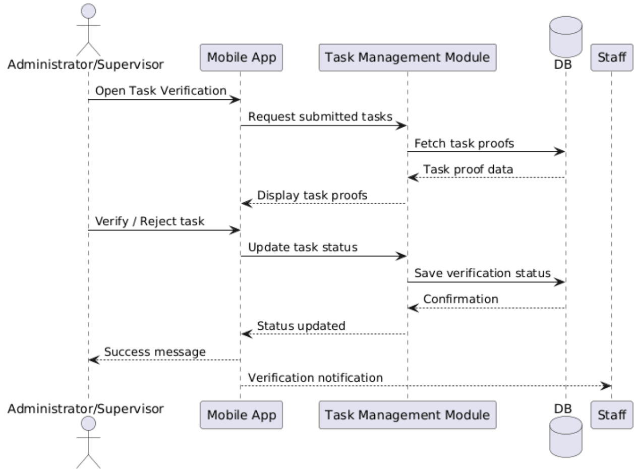
Figure 44 Sequence Diagram for Verify Task
