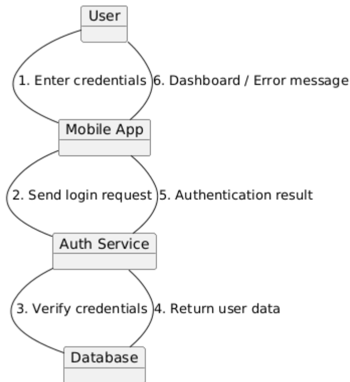
Figure 49 Collaboration Diagram For Login Process
