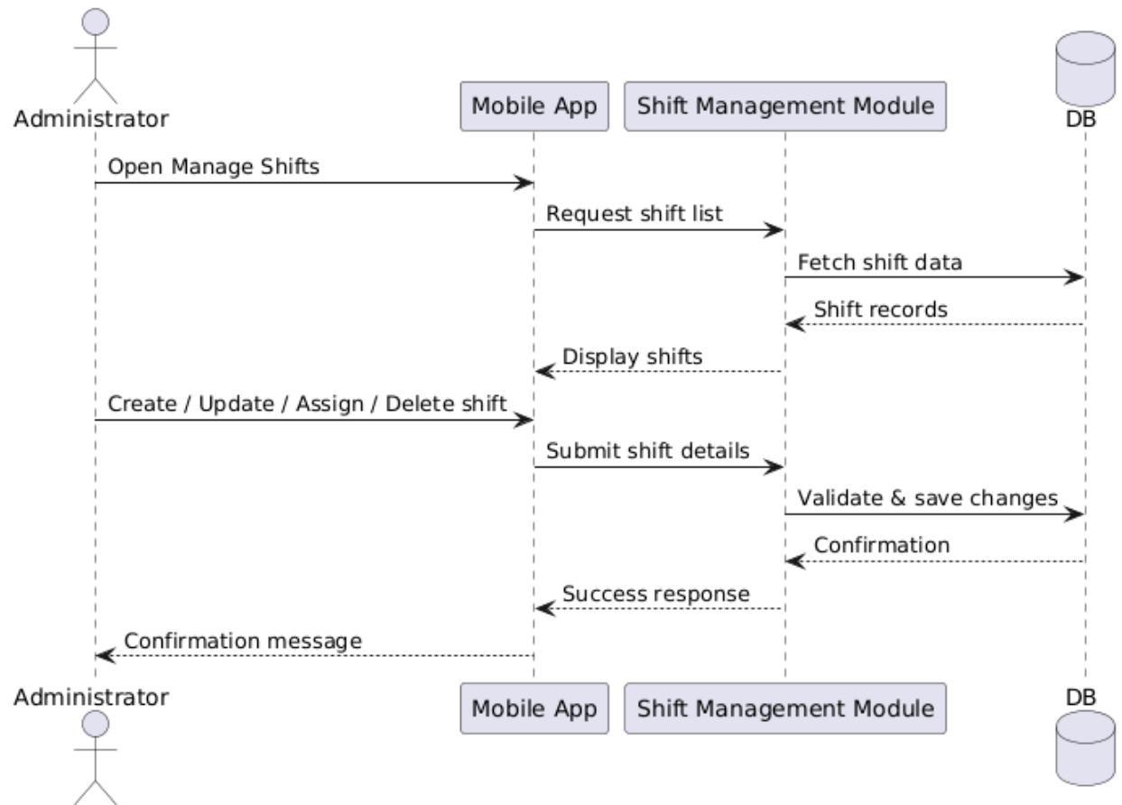
Figure 40 Sequence Diagram for Manage Shifts
