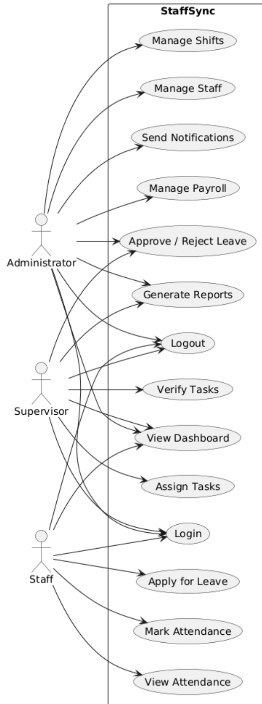
Figure 1 Use Case Diagram
