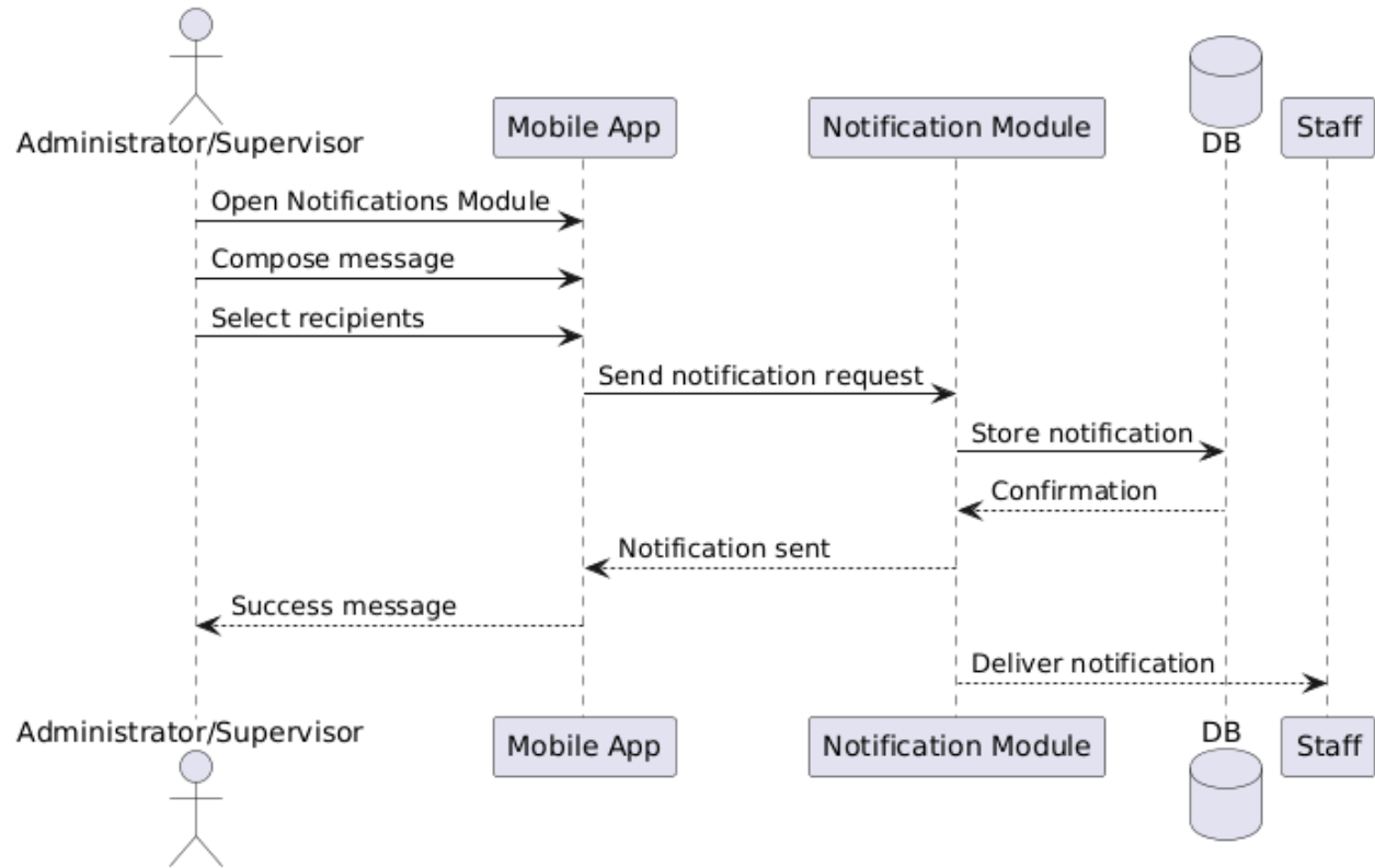
Figure 47 Sequence Diagram for Send Notifications
