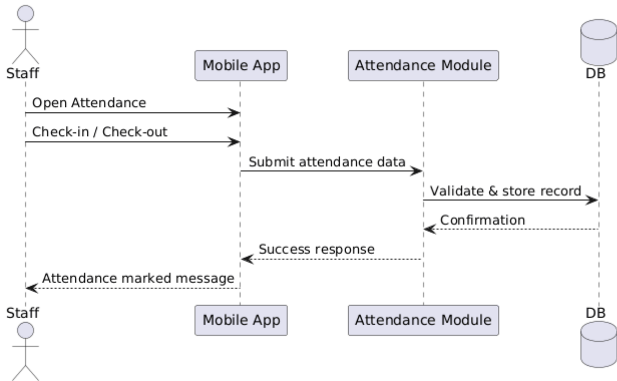
Figure 38 Sequence Diagram for Mark Attendance
