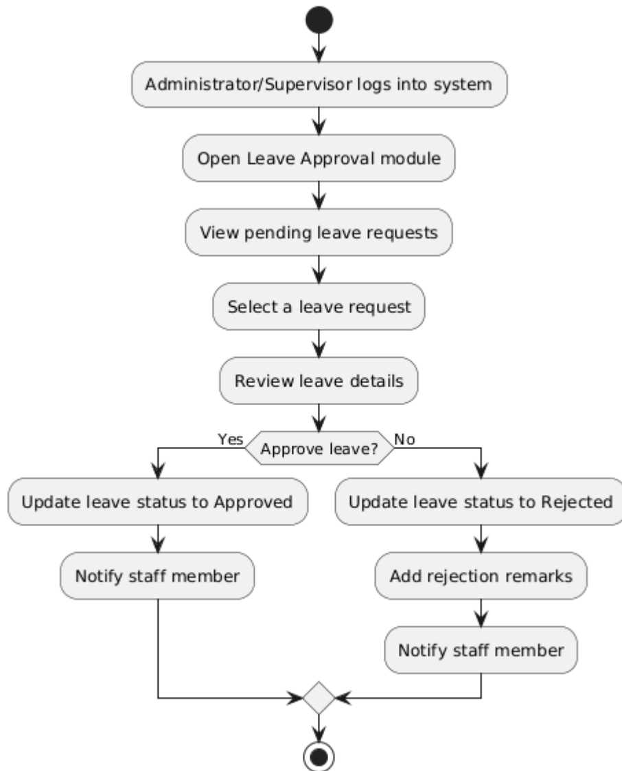
Figure 28 Activity Diagram 8: Approve / Reject Leave
