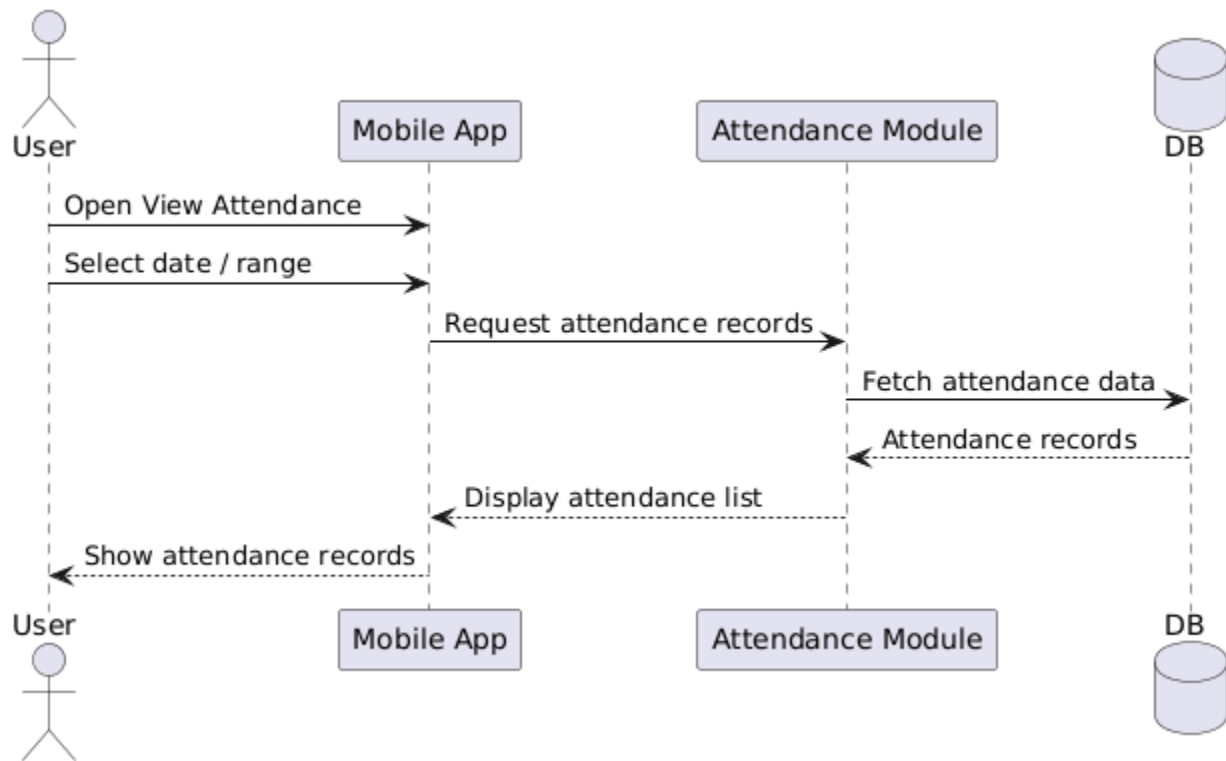
Figure 39 Sequence Diagram for View Attendance
