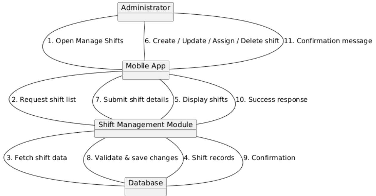
Figure 54 Collaboration Diagram for Manage Shift
