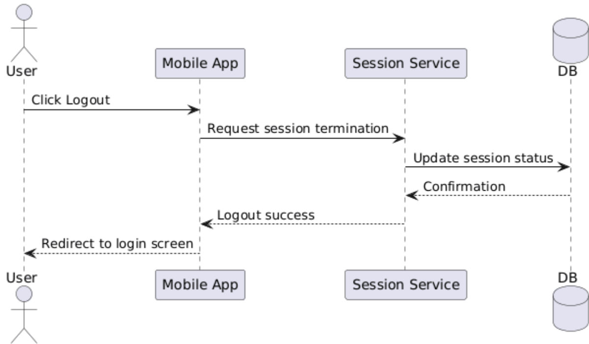
Figure 36 Sequence Diagram for Logout Process
