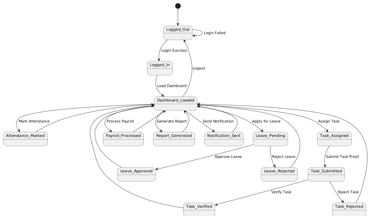
Figure 64 State Transition Diagram
