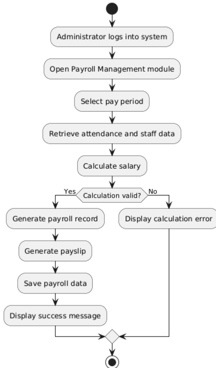
Figure 31 Activity Diagram – Manage Payroll
