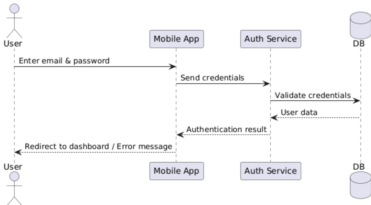
Figure 35 Sequence Diagram for Login Process
