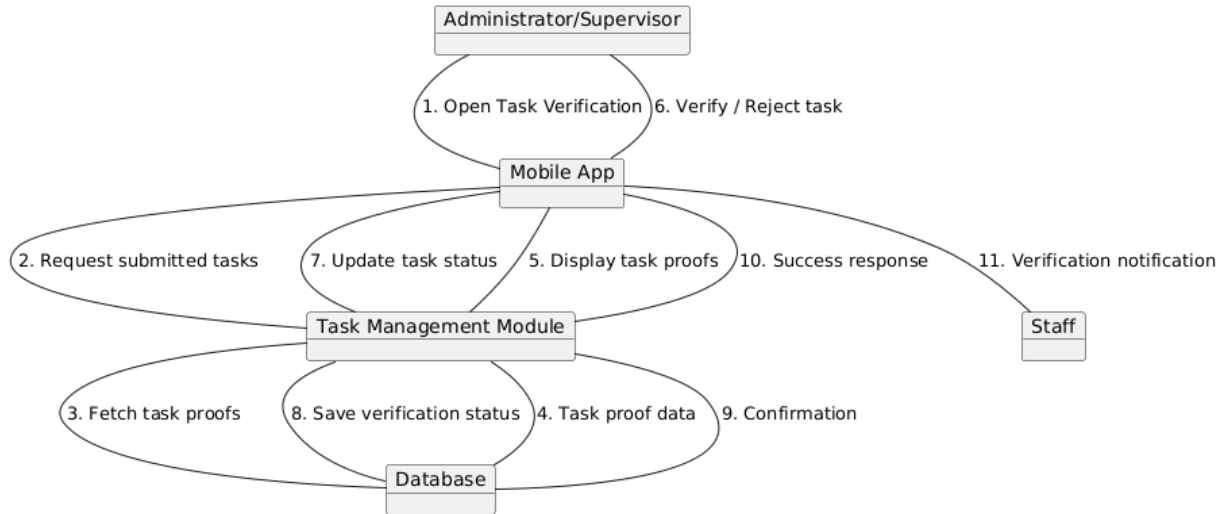
Figure 58 Collaboration Diagram for Verify Task
