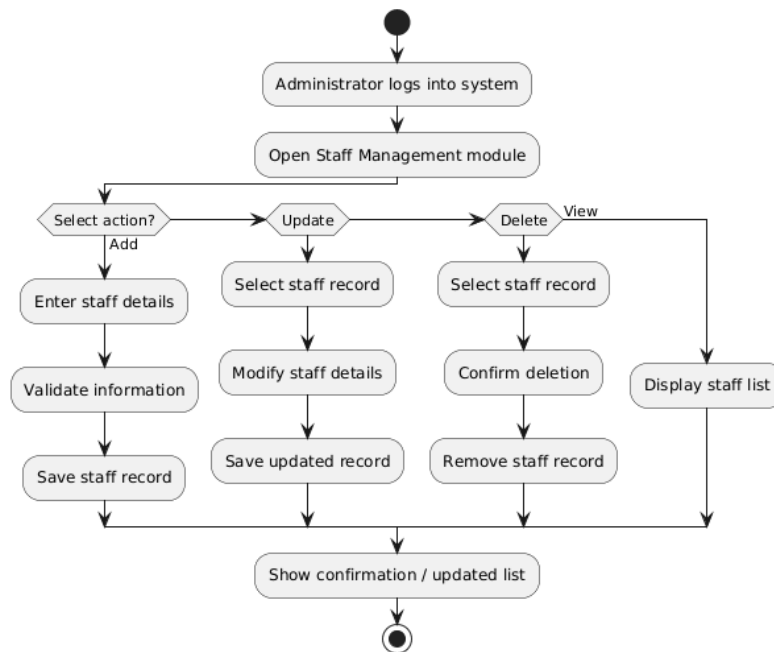
Figure 23 Activity Diagram – Manage Staff
