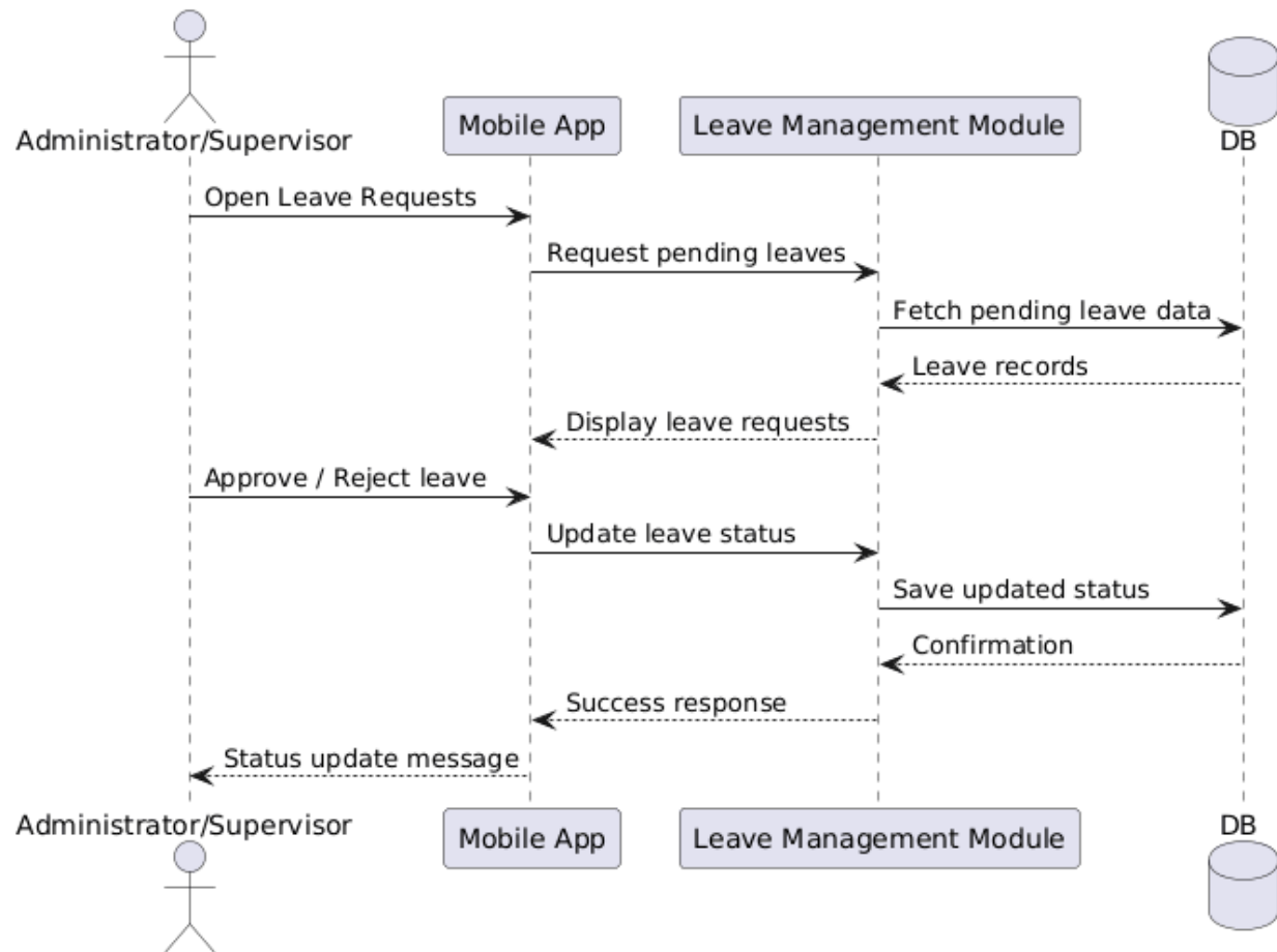
Figure 42 Sequence Diagram for Approve / Reject Leave
