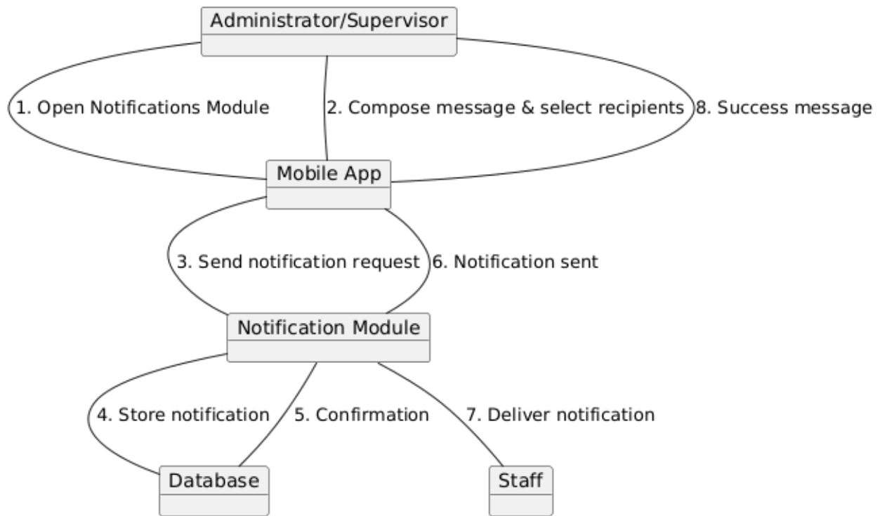
Figure 61 Collaboration Diagram for Sending Notifications
