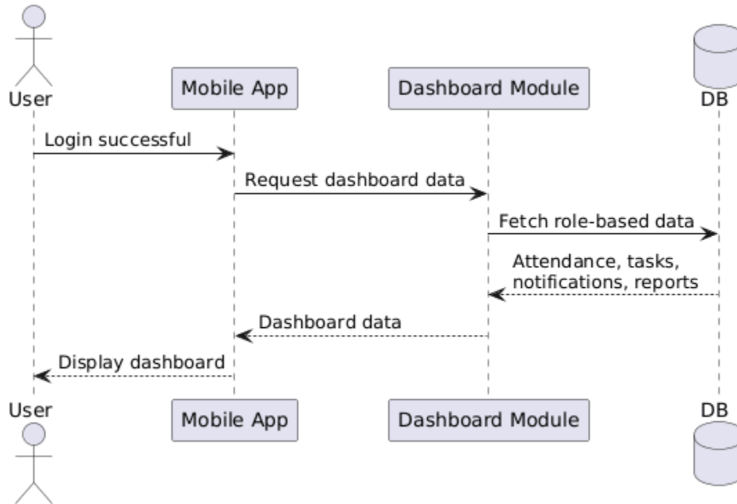
Figure 48 Sequence Diagram for View Dashboard
