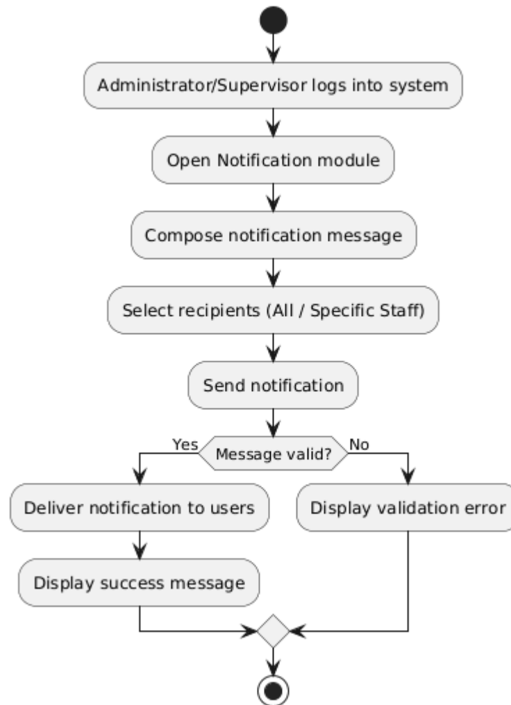
Figure 33 Activity Diagram – Send Notifications
