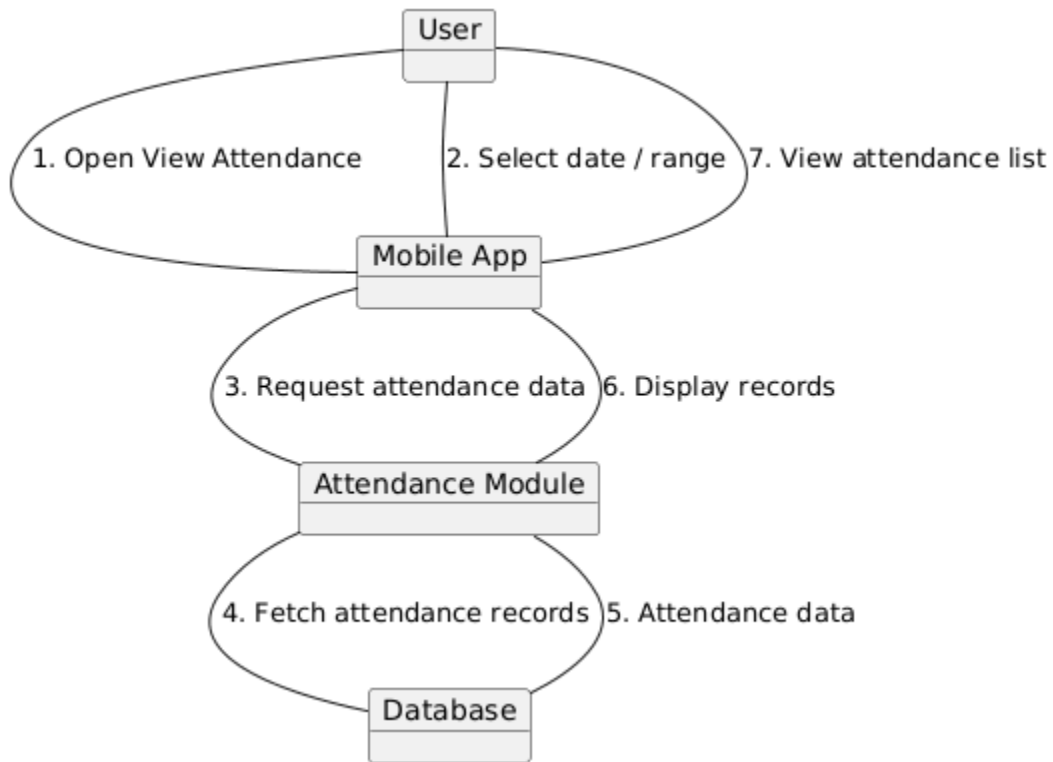
Figure 53 Collaboration Diagram for View Attendance
