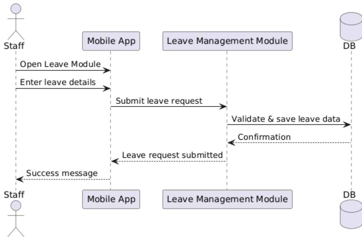
Figure 41 Sequence Diagram for Apply For Leave
