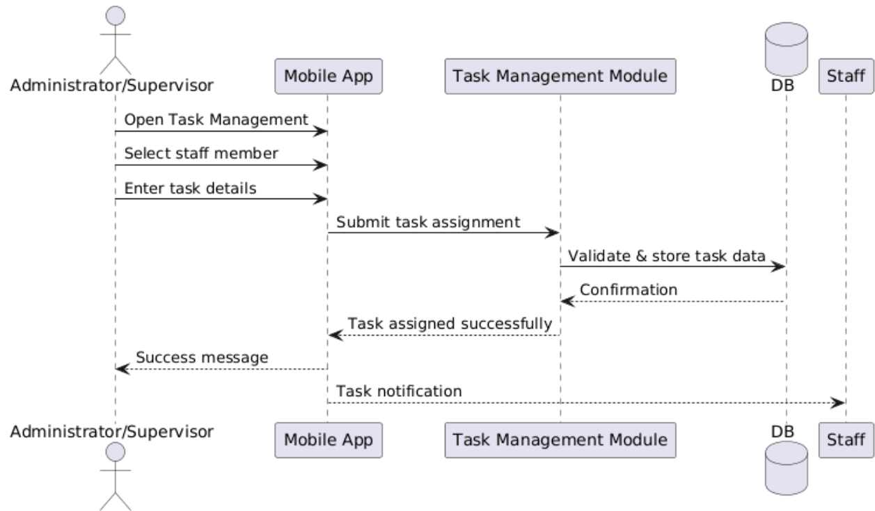
Figure 43 Sequence Diagram for Assign Task
