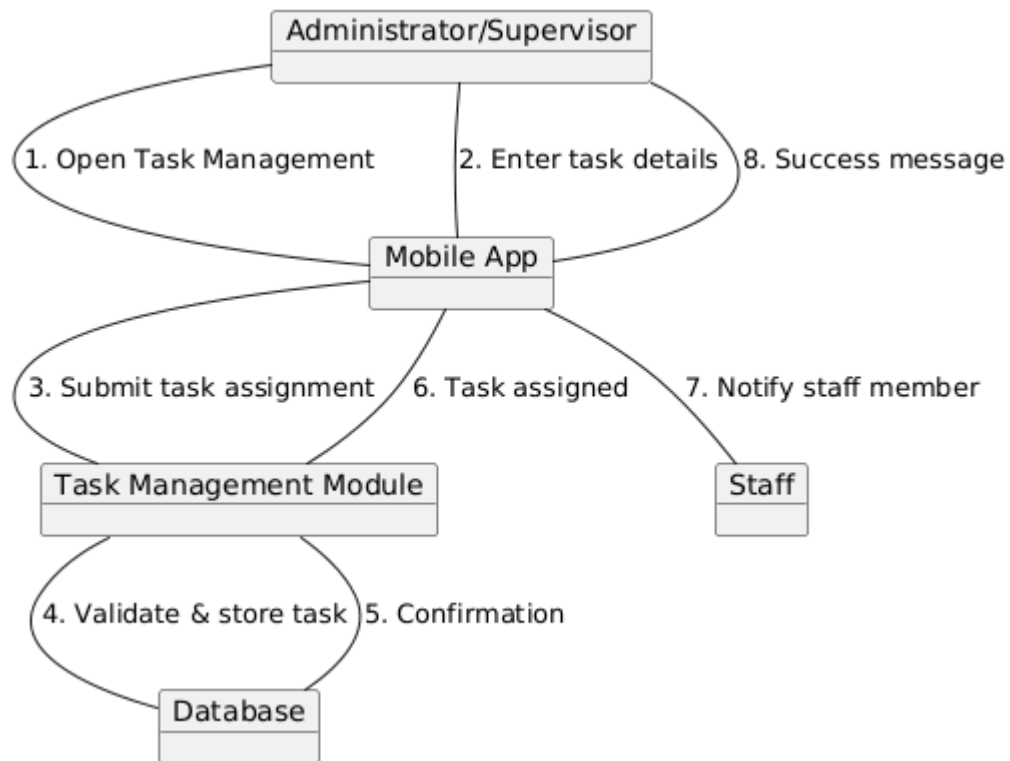
Figure 57 Collaboration Diagram for Assign Task
