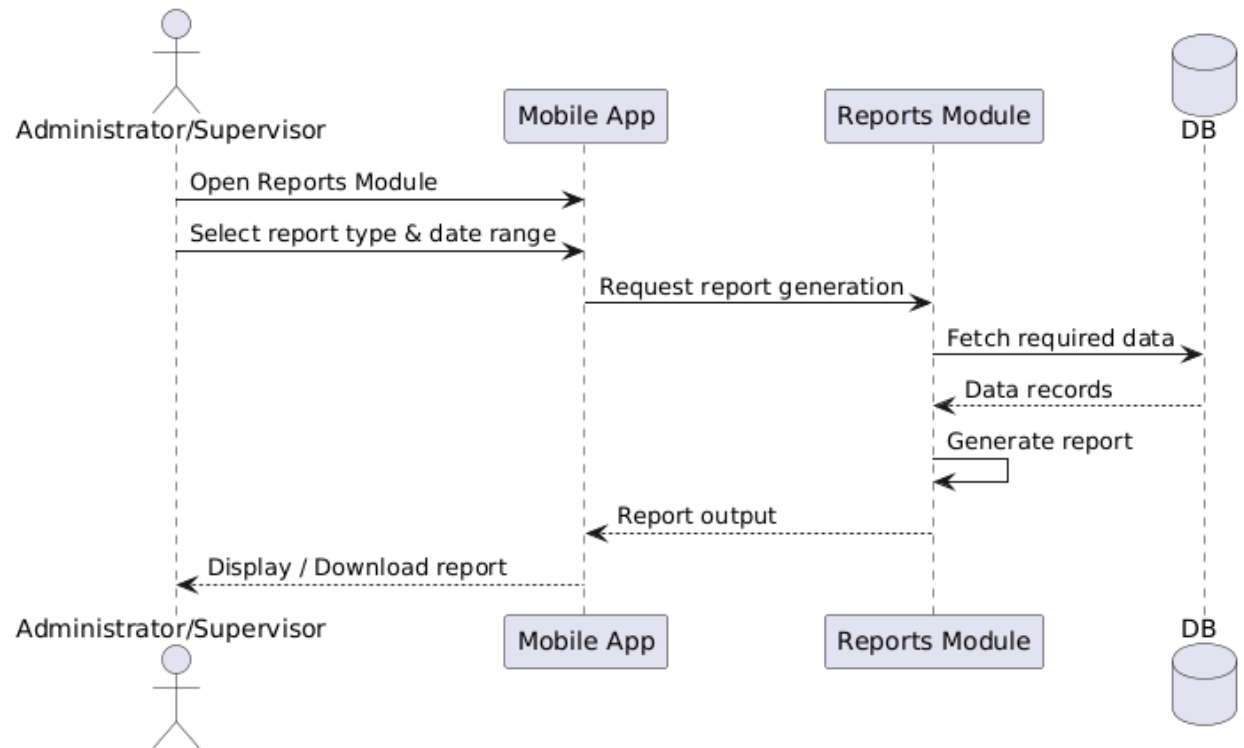
Figure 46 Sequence Diagram for Generate Reports
