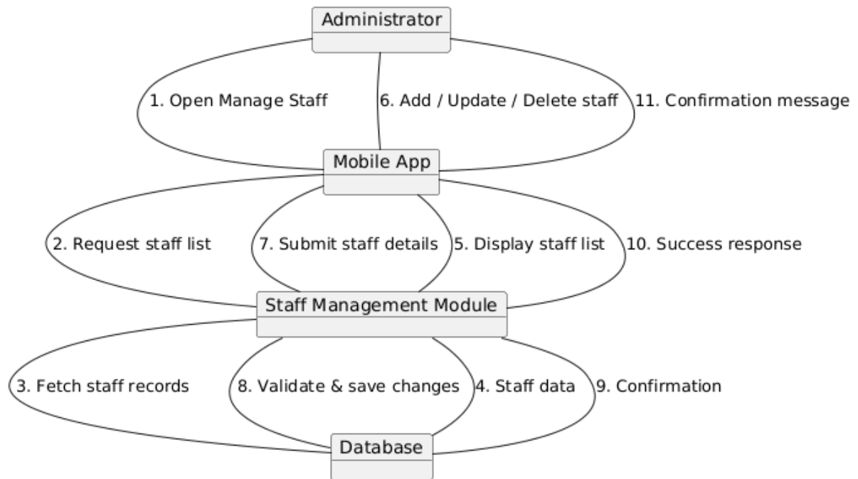
Figure 51 Collaboration Diagram For Manage staff
