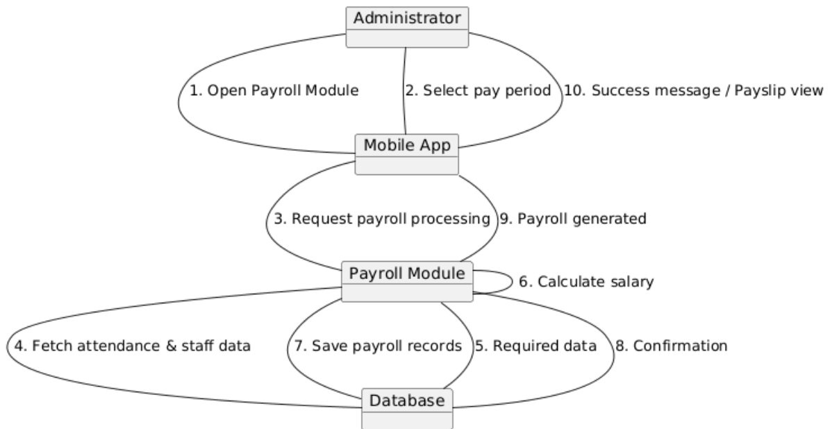
Figure 59 Collaboration Diagram for Manage Payroll
