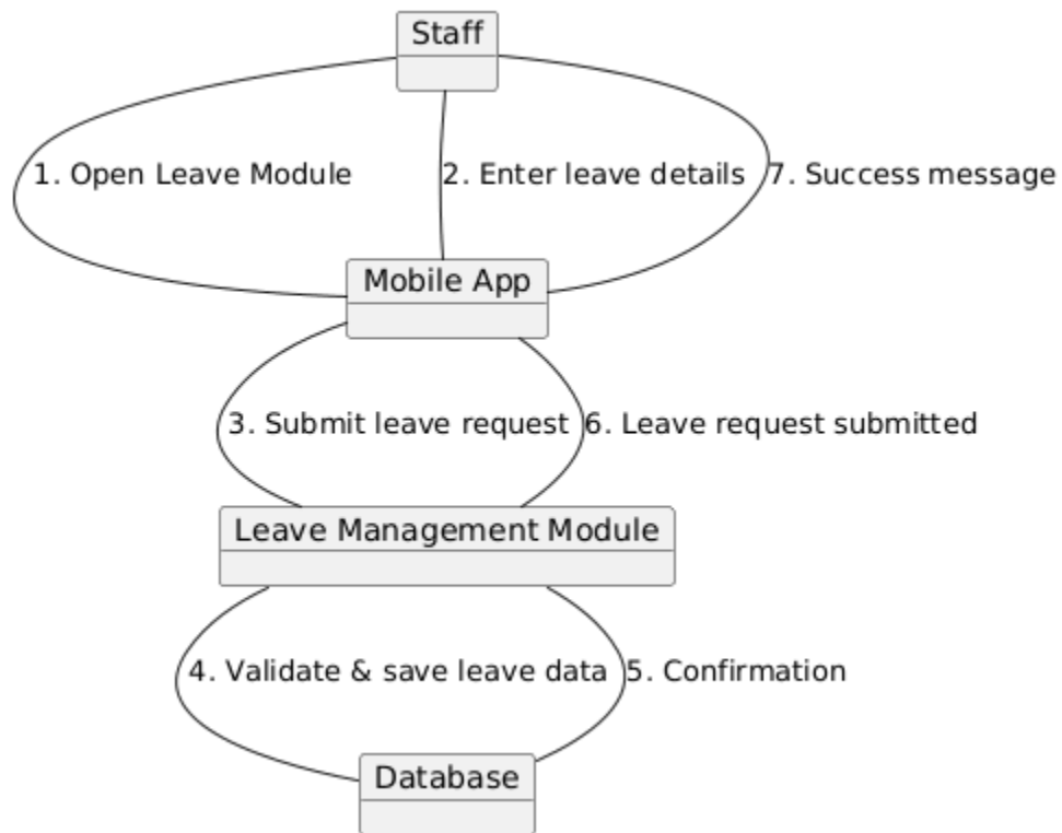
Figure 55 Collaboration Diagram for Apply Leave
